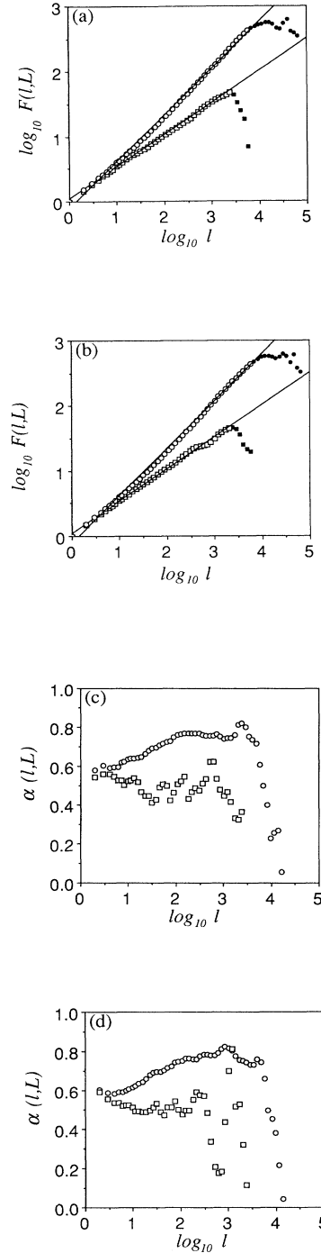
FIG. 3. Double-logarithmic plots of fluctuation F(l, L) vs nucleotide distance l [(a) and (b)] for the sequences presented in Fig. 1 and the successive slopes of these plots \alpha(l, L) vs \log_{10} l [(c) and (d)]. The actual DNA sequences are presented in (a) and (c): the entire HUMHBB sequence ( \circ ) and LINE-1c sequence ( \square ). The slopes for the linear fits are 0.72 and 0.49, respectively. The Lévy model sequences are presented in (b) and (d): the entire Lévy-walk sequence of Fig. 1(c) ( \circ ), a segment of this walk of Fig. 1(d) ( \square ). The slopes for the linear fits are 0.73 and 0.49, respectively. The solid circles and solid squares in (a) and (b) are data omitted in linear regression fit.
