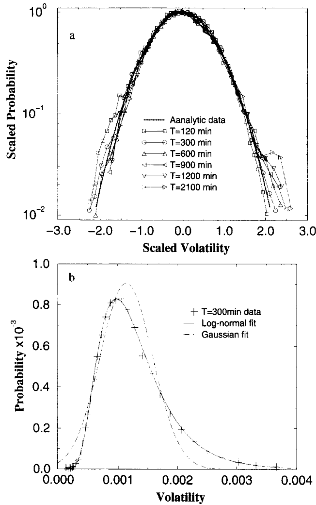
Fig. 2. (a) The volatility distribution for different window sizes T in scaled form, \sqrt{\mu} \exp(a + \mu/4) P(v_T) as a function of (\ln(v_T) - a)/\sqrt{\pi\mu} , where a and \mu are the mean and the width on a logarithmic scale. By the scaling, all curves collapse to the log-normal form with a = 0 and \mu = -1 , \exp(-(\ln x)^2) (dotted line). (b) Comparison of the best log-normal and Gaussian fits for the 300 min data.
