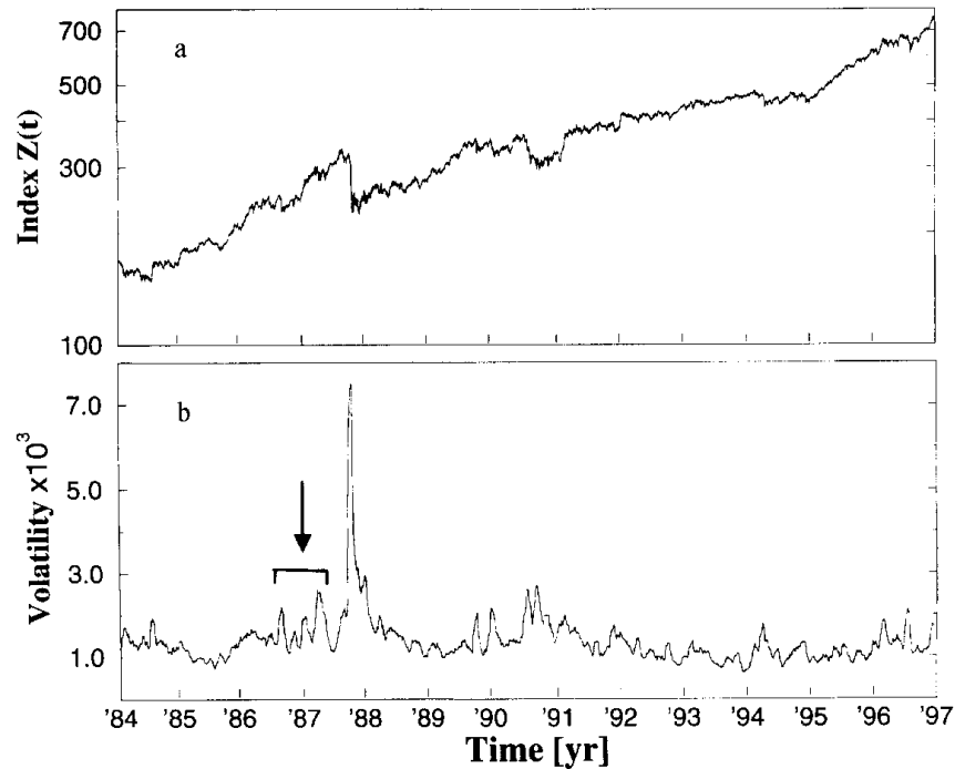
Fig. 1. (a) The S&P500 index Z(t) for 1 Jan. 1984–31 Dec. 1996. Note the large fluctuations, such as that on 19 Oct. 1987 (“black Monday”). (b) Volatility v_T(t) with T = 8190 min (1 mon) and time lag 30 min. The precursors of the 1987 crash are indicated by an arrow.
