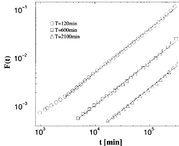
Fig. 3. The fluctuation F(t) of volatility v_T(t) with T = 120, 600, and 2100 min, calculated using detrended fluctuation analysis (DFA) [15]. To implement the DFA method, we integrate v_T(t) once; then we determine the fluctuations F(t) of the integrated signal around the best linear fit in a time window of size t . The lines are the best power-law fits with exponents \alpha = 0.91, 0.89, and 0.91 .
