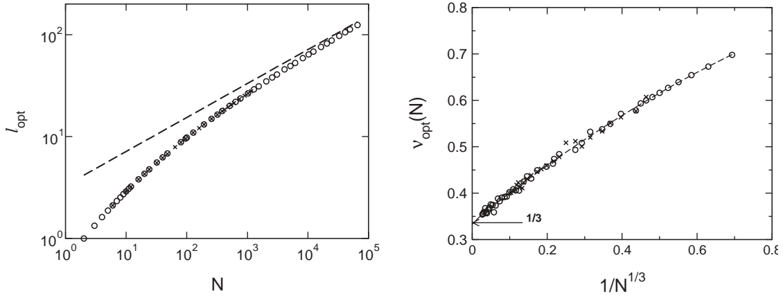
Fig. 2. Left: Plot of \ell_{\text{opt}} as a function of N in double logarithmic scale for the optimal path length in strong disorder using the two numerical methods discussed in the text: (i) results obtained using the “bombing” approach ( \circ ) and (ii) results obtained using the ultrametric approach ( \times ). The dashed line shows the slope \frac{1}{3} . Right: Successive slopes v_{\text{opt}}(N) as a function of 1/N^{1/3} for the optimal path length in strong disorder using the two methods described in the text. The symbols denote the same as in Fig. 2. The dashed line is the quadratic fitting of the results showing that the extrapolated value of the effective exponent in the limit N \rightarrow \infty approaches \frac{1}{3} . This result coincides with our theoretical value v_{\text{opt}} = \frac{1}{3} asymptotically.
