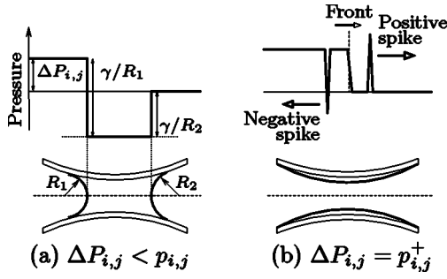
FIG. 9. Pressure along the axis of a liquid bridge in branch (i,j) when \Delta P_{i,j} is just above p_{i,j} , the liquid bridge breaks, a pair of sound waves (“crackles”) are generated, and the pressure front propagates downstream.
