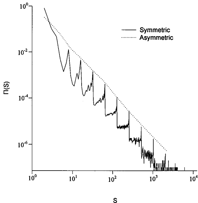
FIG. 4. Double logarithmic plots of the size distributions \Pi(S) of all avalanches for definition B using the generation-independent distribution of P_{i,j} . Both curves are shown for the normalized-rigid 12-generation Cayley tree. The solid line is the symmetric tree with characteristic “kinks” at avalanche sizes of integral powers of 2. The dotted line represents the asymmetric tree.
