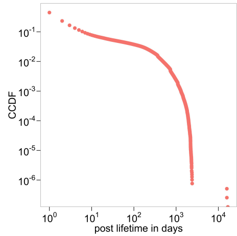
Figure 2: Complementary Cumulative Distribution Functions of the posts lifetime. The lifetime of a post is the time period between its first and its last comment.
