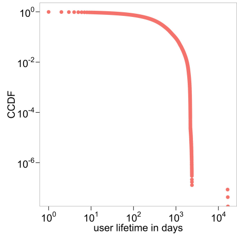
Figure 4: Complementary Cumulative Distribution Functions of the users lifetime. The lifetime of a user is the time period between their first and their last comment.
