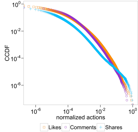
Figure 1: Complementary Cumulative Distribution Functions (CCDFs) of the number of likes, comments and shares of the posts.
