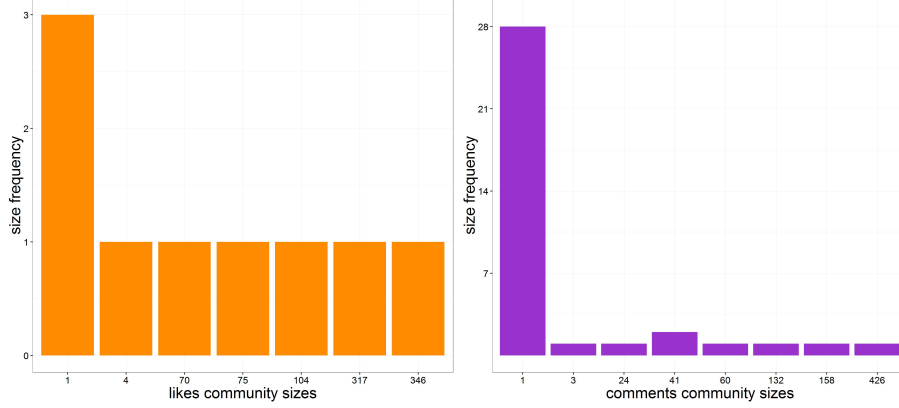
Figure 5: Community Sizes Frequency. Sizes of the Fast Greedy communities of G_l^p on the left, and G_c^p on the right.
