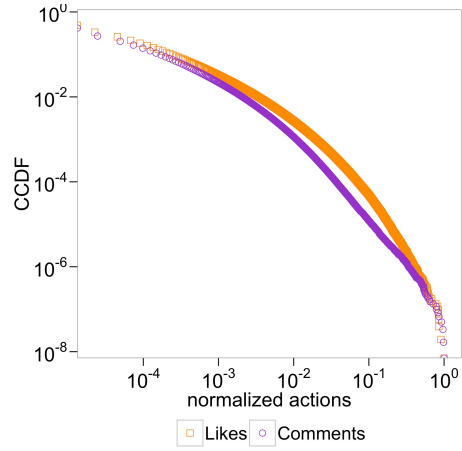
Figure 3: Complementary Cumulative Distribution Functions of the number of likes and comments of the users. For the likes calculation, a sample of 51 million users was used (518 million likes).
