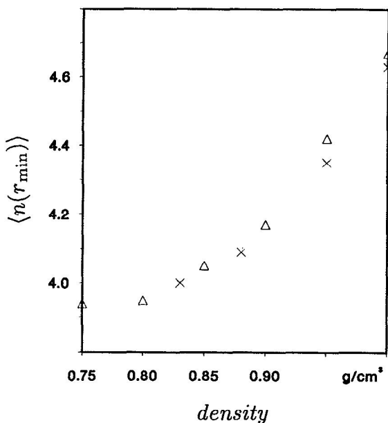
FIG. 2. Density dependence in ST2 water at 273 K (triangles) and 235 K (crosses) for the number of neighbors inside a shell of 3.3 Å. Here the number of neighbors is calculate using quenched configurations.
