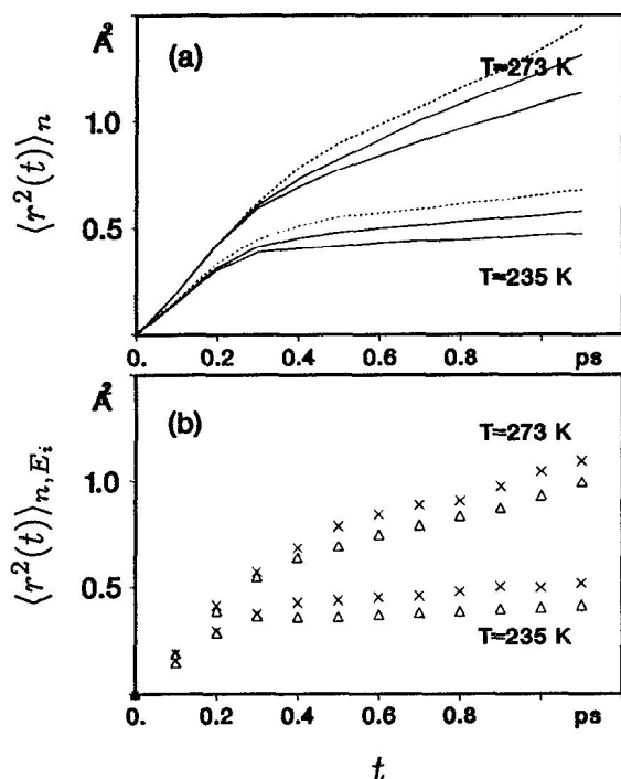
FIG. 9. (a) Mean square displacement \langle r^2(t) \rangle_n for groups of molecules with number of neighbors n equal to four (full line), five (dashed line), and six (dotted) for T=235 and 273 K. (b) Mean square displacement \langle r^2(t) \rangle_{n,E_i} for molecules with four (triangles) and five (crosses) neighbors and binding energy E_i between 110 and 115 kJ/mol.
