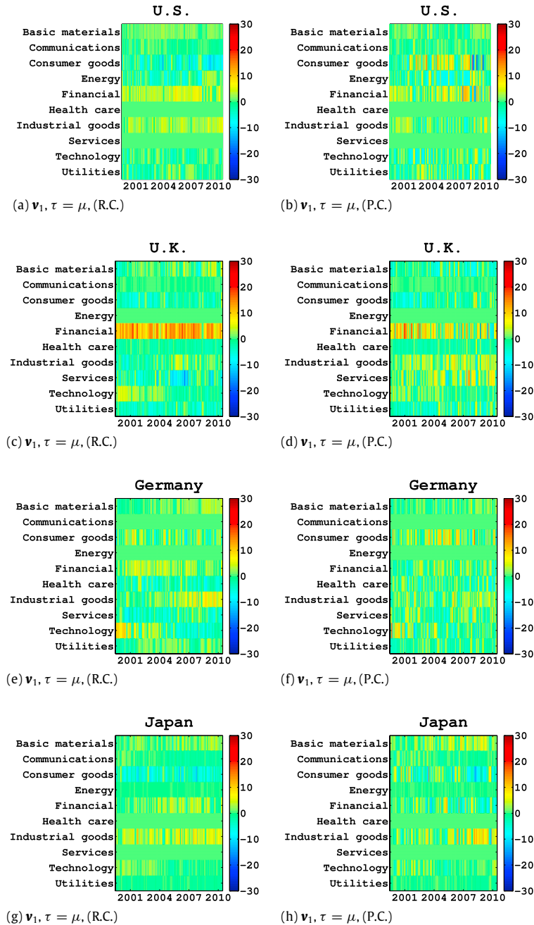
Fig. B.10. The monthly based SDR calculated from \mathbf{v}_1 with \tau = \mu for raw and partial correlations, for the US (a, b), UK (c, d), Germany (e, f), and Japanese (g, h) stock markets.
