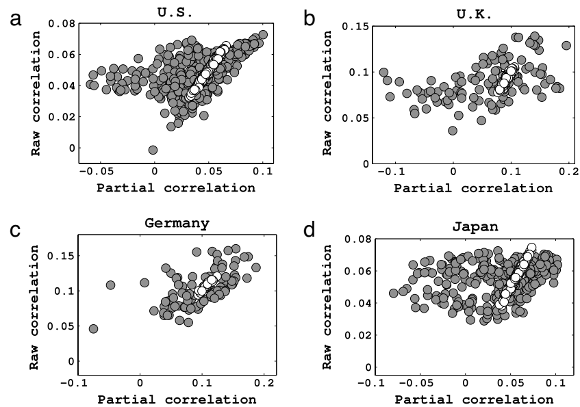
Fig. 2. The weight of components of eigenvector \mathbf{v}_1 from the US (a), UK (b), Germany (c) and Japanese (d) stock markets. The x-axis indicates the value of components of \mathbf{v}_1 derived from partial correlation and y-axis indicates the value of components for raw correlation for corresponding stocks. Gray circles indicate components of \mathbf{v}_1 from each stock, and white circles are components of \mathbf{v}_1 from random data.
