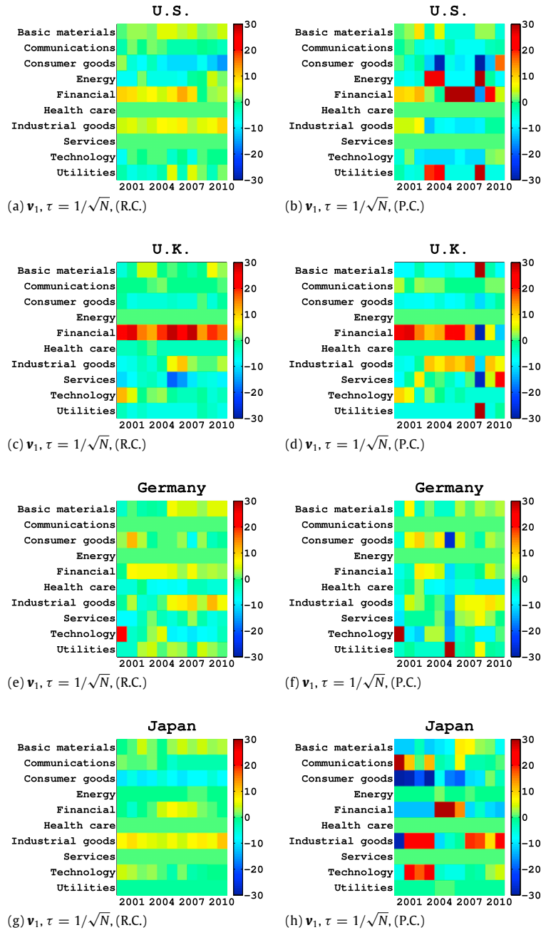
Fig. 3. Yearly based SDR analysis obtained from the largest eigenvector v_1 for the raws and partial correlations of US (a, b), UK (c, d), Germany (e, f), and Japanese (g, h) stock markets. The threshold is given as \tau = 1/\sqrt{N} .
