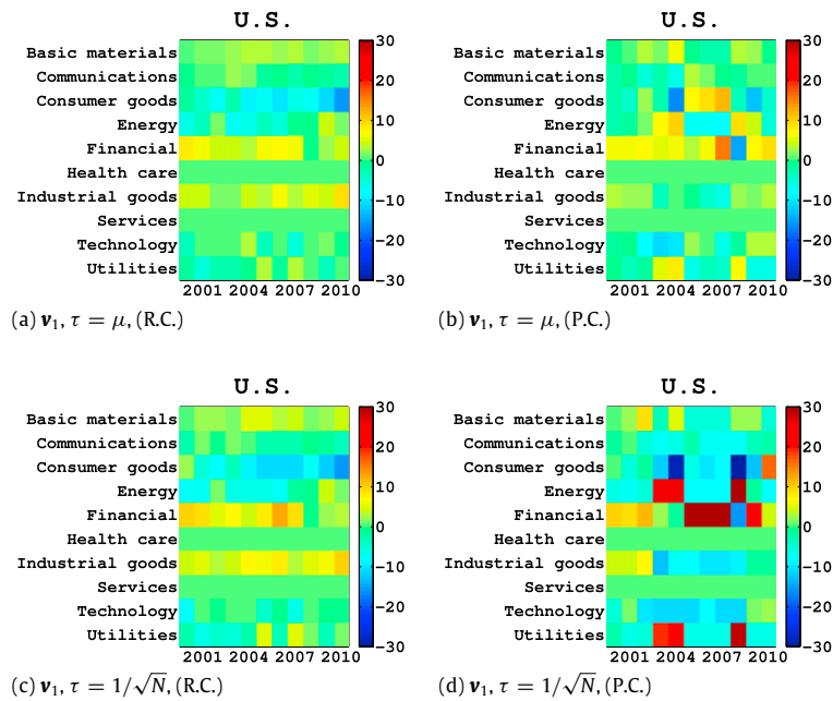
Fig. B.8. The yearly based SDR calculated from v_1 for the US stock market for different thresholds and for the first and second largest eigenvectors: (a) SDR calculated from v_1 and \tau = \mu for raw correlations; (b) SDR calculated from v_1 and \tau = \mu for partial correlations; (c) SDR calculated from v_1 and \tau = 1/\sqrt{N} for raw correlations; and (d) SDR calculated from v_1 and \tau = 1/\sqrt{N} for partial correlations.
