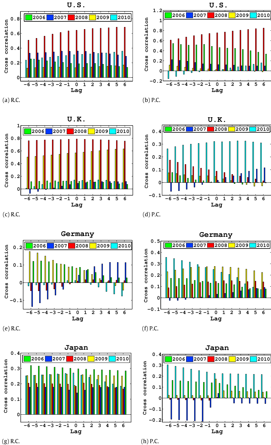
Fig. 6. Cross correlation function (XCF) between the SDR calculated for the financial sector, -\Phi_5 , and VIX by monthly basis for each year using raw and partial correlation, for the US (a, b), UK (c, d), Germany (e, f), and Japanese (g, h) stock market.
