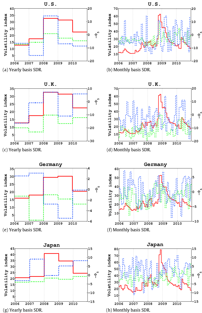
Fig. 5. The comparison of Financial sector based SDR and VIX for the period of 2006–2010, on a yearly and monthly based time horizon for the US (a, b), UK (c, d), Germany (e, f), and Japanese (g, h) stock markets. The red line corresponds to the VIX index on either yearly or monthly time horizon, and green and blue dashed lines correspond to dynamical change of -\phi_5 , which expresses deactivation of SDR for financial sector using v_1 for raw and partial correlation, respectively. The left y-axis displays the value of volatility index and the right y-axis displays the value of -\phi_5 . (For interpretation of the references to color in this figure legend, the reader is referred to the web version of this article.)
