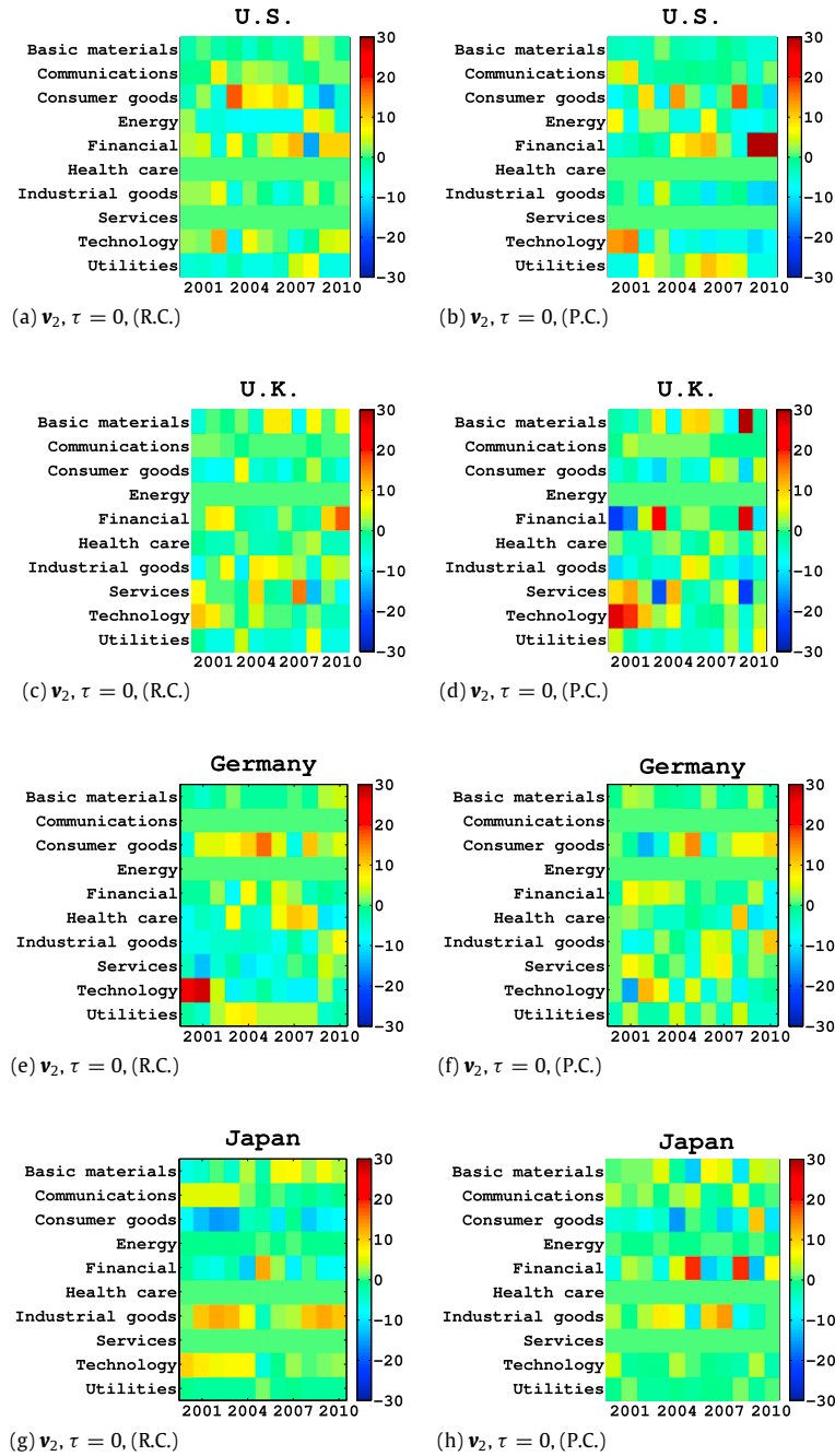
Fig. C.11. The yearly based SDR calculated from \mathbf{v}_2 with \tau = 0 for both raw and partial correlations for the US (a, b), UK (c, d), Germany (e, f), and Japanese (g, h) stock markets.
