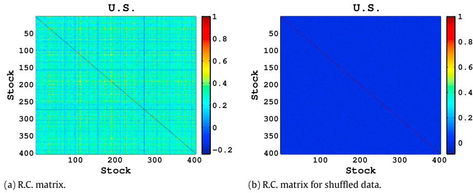
Fig. A.7. Stock raw correlation matrix for the US market, calculated from empirical data (a) and from the random ally shuffled time series (b), using the same color code. (For interpretation of the references to color in this figure legend, the reader is referred to the web version of this article.)
