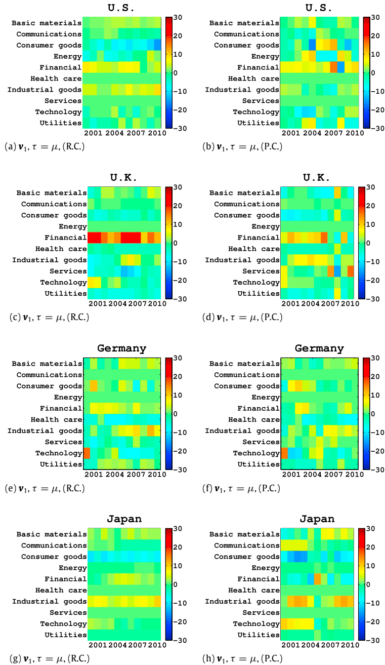
Fig. B.9. The yearly based SDR calculated from \mathbf{v}_1 with \tau = \mu for raw and partial correlations, for the US (a, b), UK (c, d), Germany (e, f), and Japanese (g, h) stock markets.
