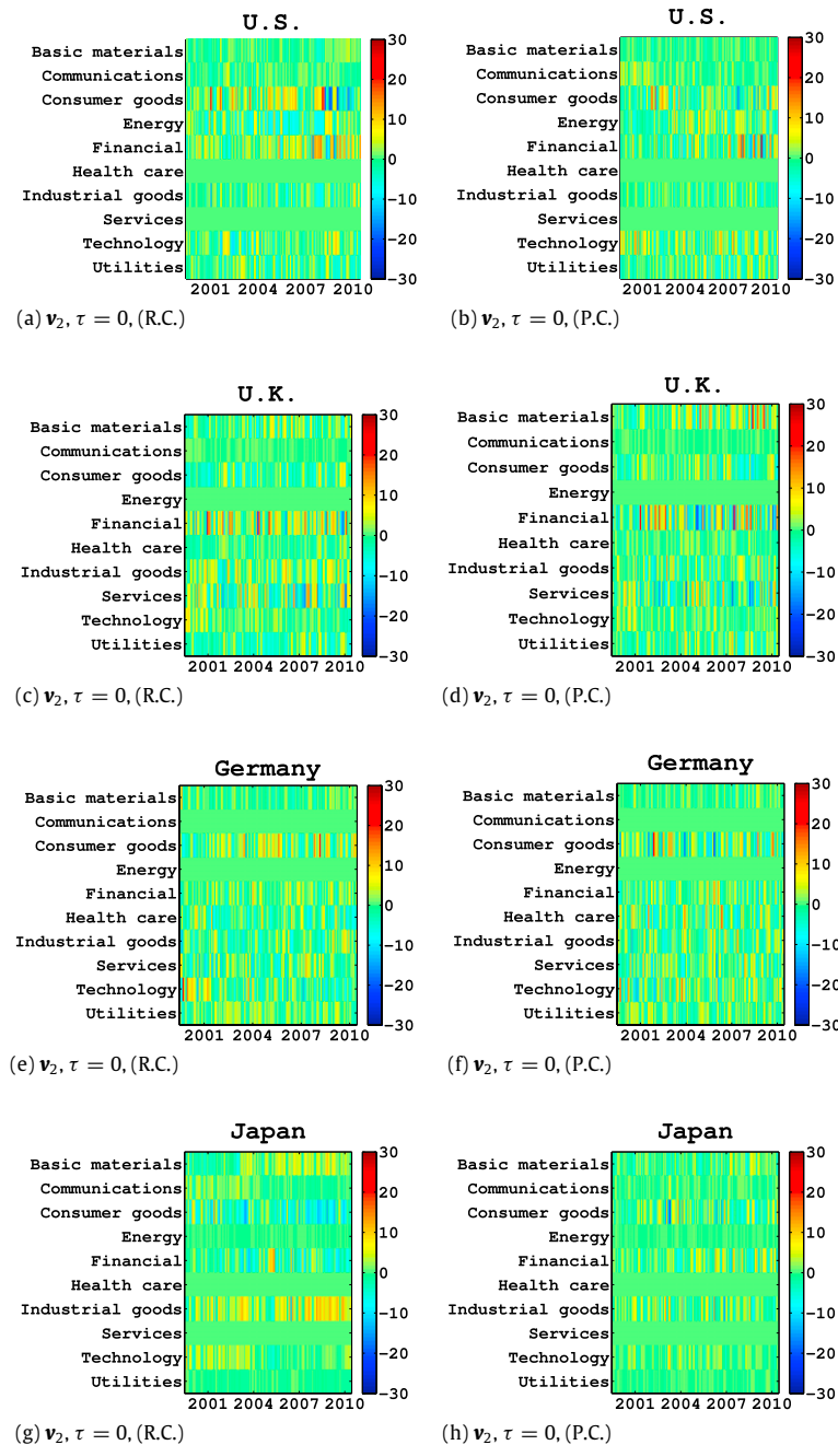
Fig. C.12. The monthly based SDR calculated from v_2 with \tau = 0 for both raw and partial correlations for the US (a, b), UK (c, d), Germany (e, f), and Japanese (g, h) stock markets.
