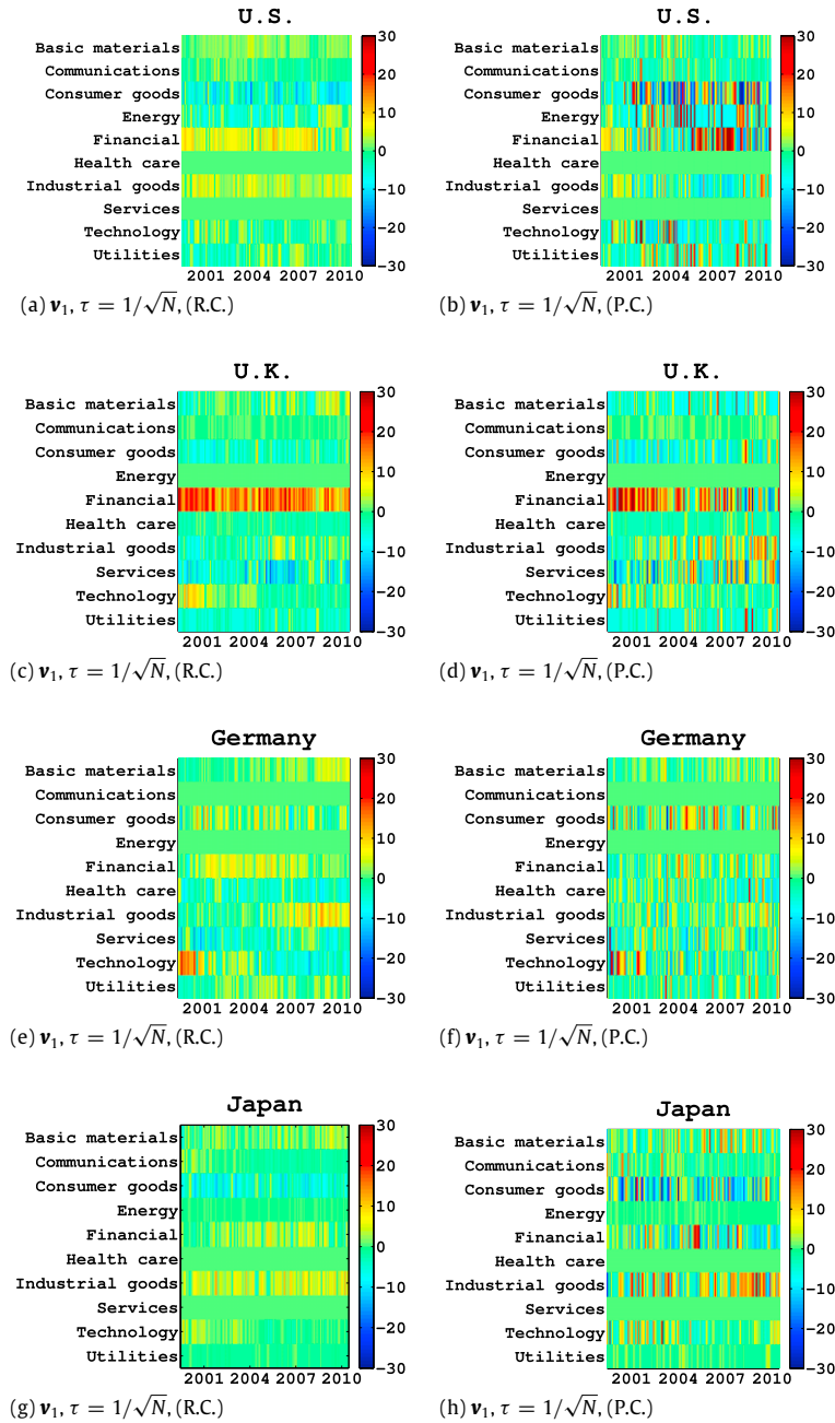
Fig. 4. Monthly based SDR analysis for the raw and partial correlations of the US (a, b), UK (c, d), Germany (e, f), and Japanese (g, h) stock markets. The dominance of the Financial sector is observed in both US and UK stock markets, but not in the German and Japanese stock markets. Furthermore, the monthly based SDR analysis highlights changes in market structure, emphasizing changes that led up to the 2008 financial crisis.
