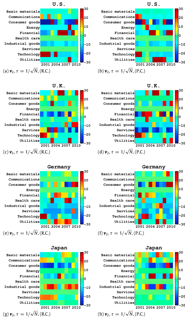
Fig. C.13. The yearly based SDR calculated from \mathbf{v}_2 with \tau = 1/\sqrt{N} for both raw and partial correlations for the US (a, b), UK (c, d), Germany (e, f), and Japanese (g, h) stock markets.
