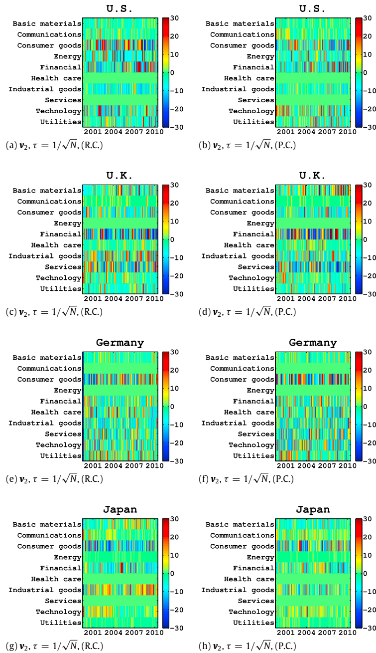
Fig. C.14. The monthly based SDR calculated from \mathbf{v}_2 with \tau = 1/\sqrt{N} for both raw and partial correlations for the US (a, b), UK (c, d), Germany (e, f), and Japanese (g, h) stock markets.
