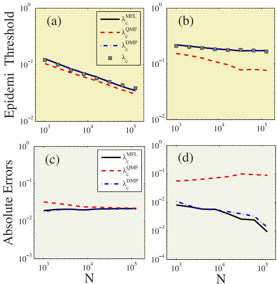
Figure 1. Predicting epidemic threshold for uncorrelated configuration networks under different network sizes. Theoretical predictions of \lambda_c^{\text{MFL}} (black solid lines), \lambda_c^{\text{QMF}} (red dashed lines), \lambda_c^{\text{DMP}} (blue dash-dotted lines) and numerical prediction (gray squares) versus network size N for degree exponent \nu_D = 2.1 (a) and \nu_D = 3.5 (b). The absolute errors between \lambda_c and \lambda_c^{\text{MFL}} (black solid lines), \lambda_c^{\text{QMF}} (red dashed lines) and \lambda_c^{\text{DMP}} (blue dash-dotted lines) versus N for \nu_D = 2.1 (c) and \nu_D = 3.5 (d).
