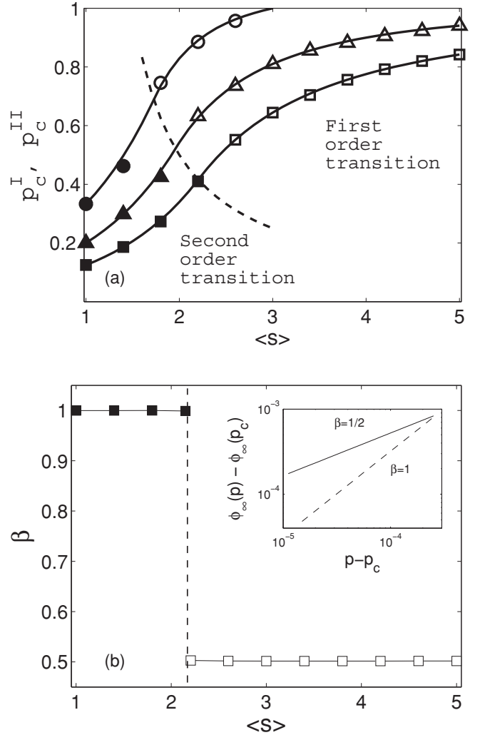
FIG. 7. (a) Theory (lines) and simulations (symbols) are compared for the values of p_c^I(\langle s \rangle) and p_c^{II}(\langle s \rangle) for ER networks with different average degree k (circles for k = 3 , triangles for k = 5 , and squares for k = 8 ). For \langle s \rangle > \langle s \rangle_c (dashed line) the network undergoes a first-order transition. The theoretical values of the transition point p_c^I(\langle s \rangle) that are calculated according to Eq. (29) are compared with simulations (open symbols) performed using the NOI method (explained in text). For \langle s \rangle < \langle s \rangle_c the network undergoes a second-order transition, and the theoretical values of the transition point p_c^{II}(\langle s \rangle) that are calculated according to Eq. (28) are compared with simulations (solid symbols) performed using the second-largest cluster method. The dashed line separating the first and second orders is obtained according to Eq. (32). (b) The size of the giant cluster \phi_{\infty} above the critical point p_c is described by \phi_{\infty}(p) - \phi_{\infty}(p_c) \sim (p - p_c)^{\beta} , as shown in the inset. The critical exponent \beta above the transition point p_c is plotted vs the average size of the dependency clusters \langle s \rangle for a network with k = 8 [compare to (a); squares]. For the region of the second-order transition, \langle s \rangle < \langle s \rangle_c , we find \beta = 1 ( \langle s \rangle_c is marked by the vertical dashed line), while for the region of the first-order transition, \langle s \rangle > \langle s \rangle_c , \beta = 1/2 .
