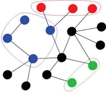
FIG. 1. (Color online) Connectivity network with dependency clusters. The edges represent connectivity relations, while the (blue, red, and green) groups surrounded by curves represent dependency relations between all the nodes of the same group (color). The dependency relations can be between very “far” nodes in the connectivity network. In the general case, the sizes of each dependency clusters follow a given distribution.
