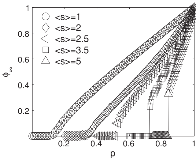
FIG. 6. The size of the giant cluster, \phi_{\infty} \equiv P_{\infty} p , vs p for ER networks ( k = 8 ) and Poisson distribution of dependency clusters with different average sizes \langle s \rangle . The symbols represent simulation results of systems of 50 000 nodes, and the solid lines show the theoretical predictions. For \langle s \rangle = 1 and 2 the network undergoes a second-order transition, while for \langle s \rangle = 2.5, 3.5 , and 5 the network undergoes a first-order transition [see Fig. 7, where the exact transition point from first- to second-order transition is shown].
